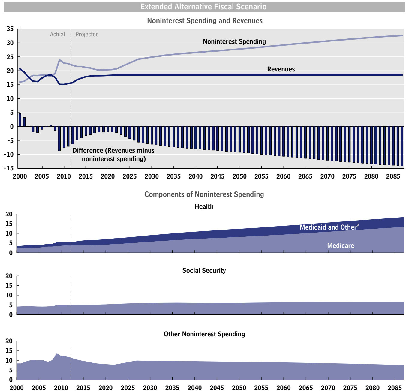
Figure B-1. Continued Noninterest Spending and Revenues Under CBO’s Long-Term Budget Scenarios Through 2087
