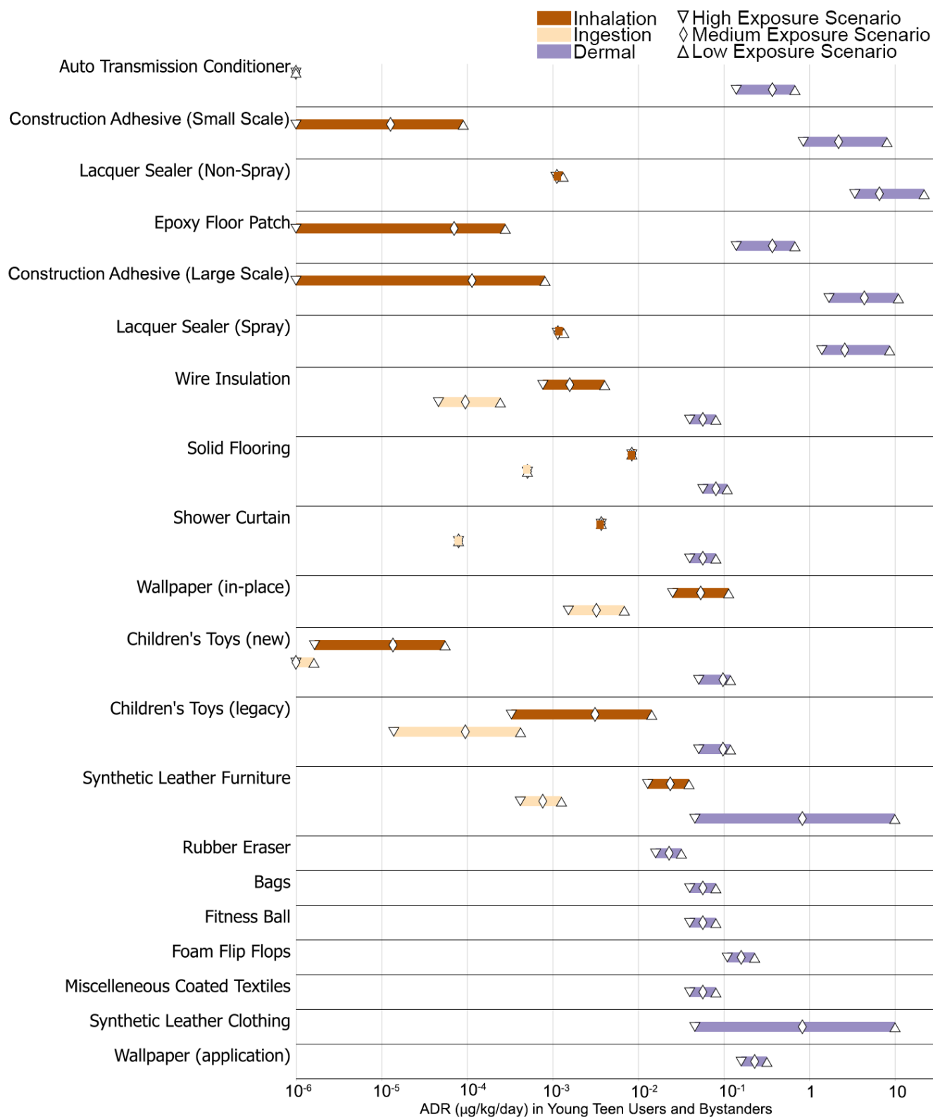
Figure 3-9. Acute Dose Rate of DIDP from Ingestion, Inhalation, and Dermal Exposure Routes for Young Teen 11–15 Years Old
