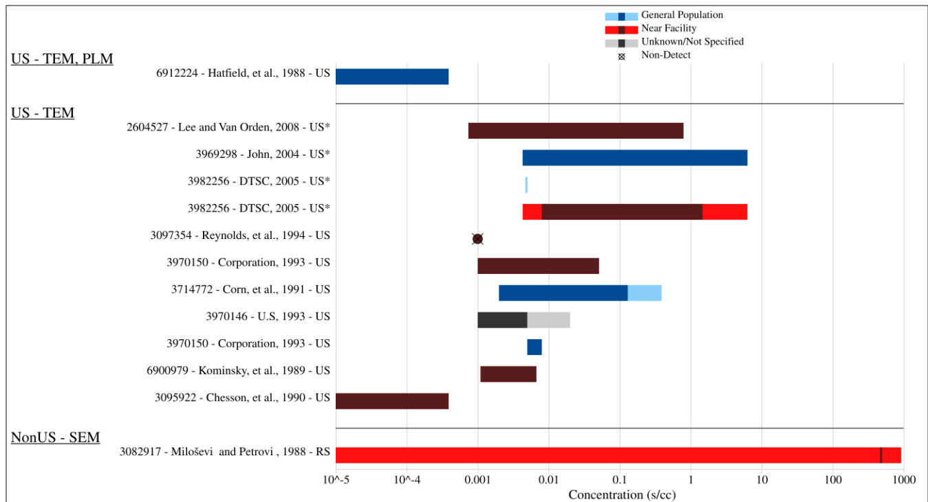
Figure_Apx F-2. Concentrations of Asbestos (s/cc) in Ambient Air from 1975 to 2008
