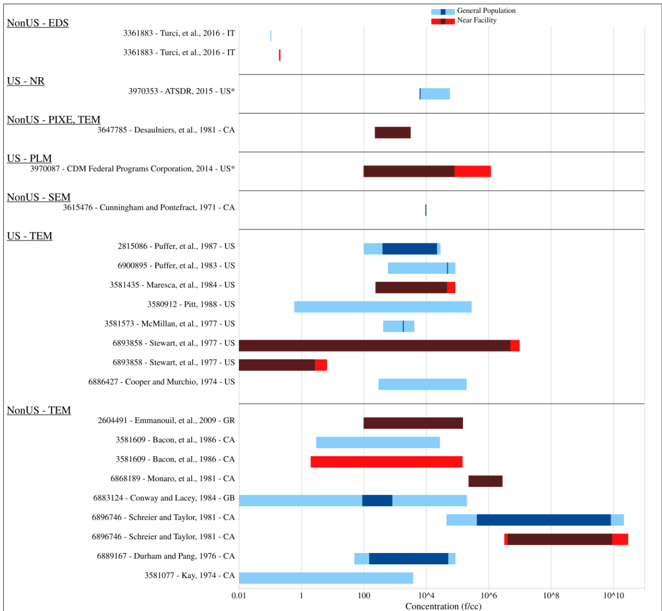
Figure_Apx F-11. Concentrations of Asbestos (f/cc) in Surface Water from 1971 to 2016
