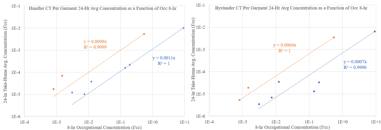
Figure 3-4. Take-Home Exposure Slope Factor Regression for Handler and Bystander
