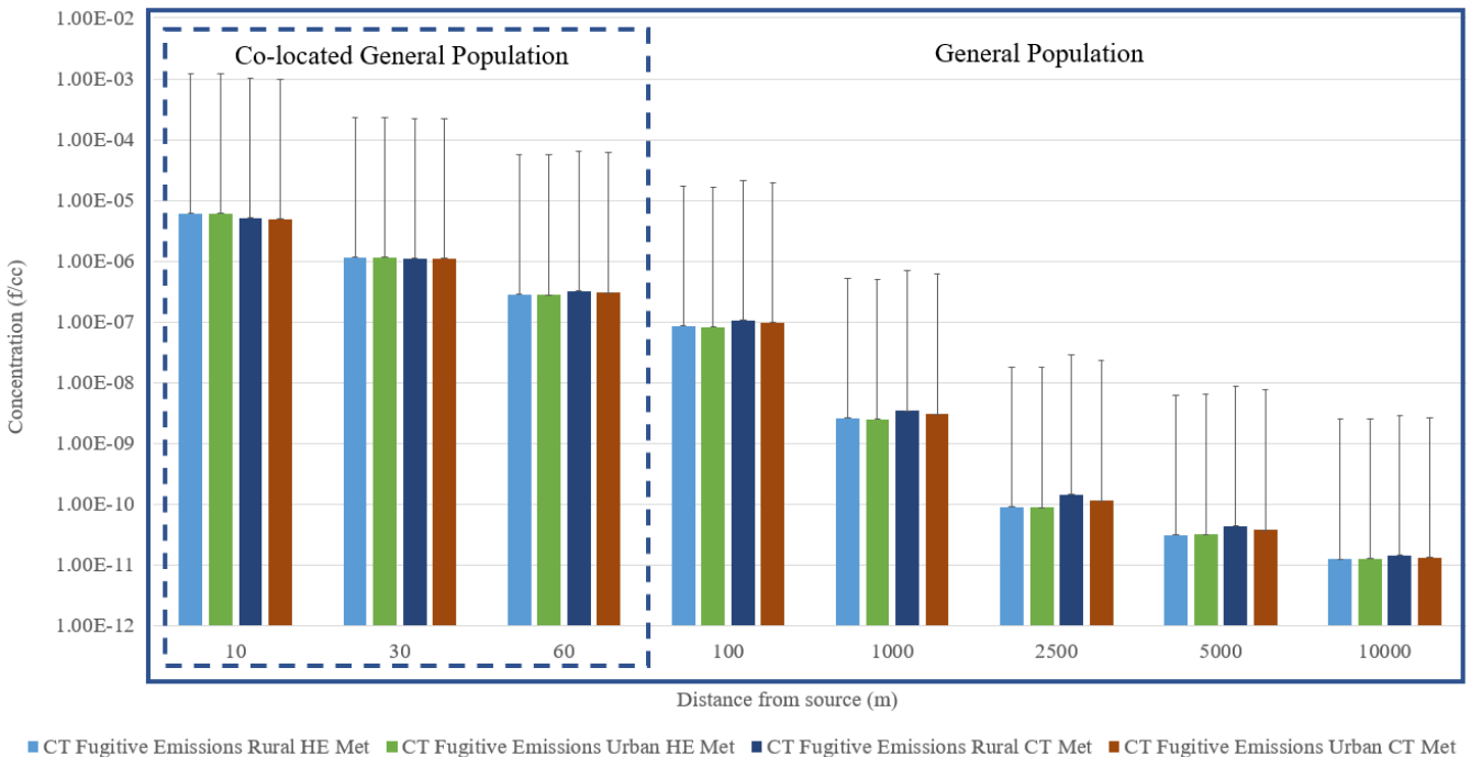
Figure_Apx F-9. Generic Annual Ambient Air Asbestos Concentrations: Handling Asbestos-Containing Building Materials During Maintenance, Renovation, and Demolition Activities
