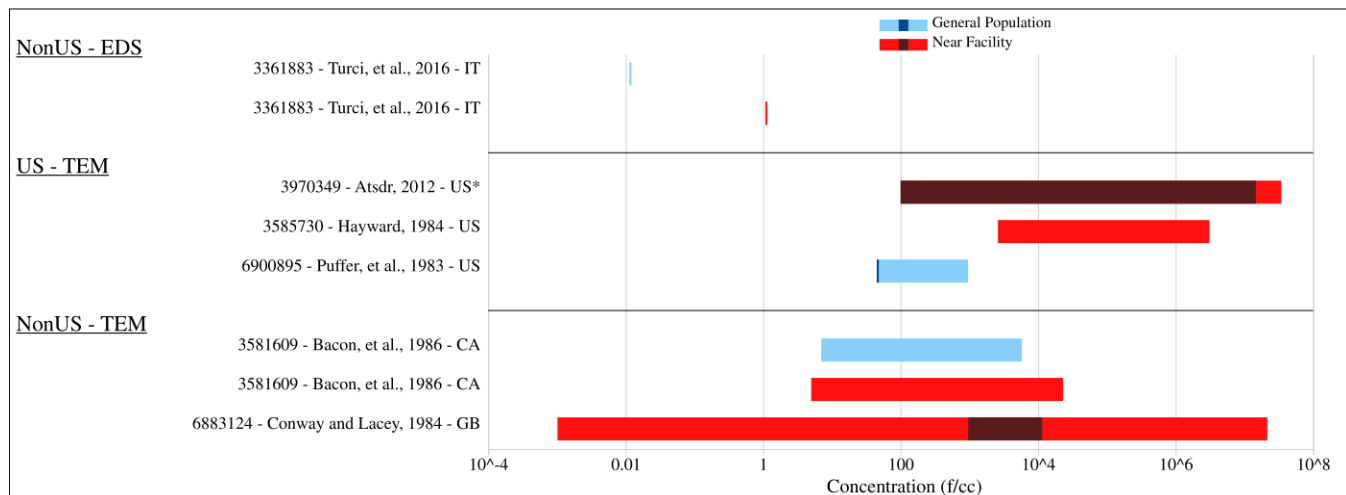
Figure_Apx F-13. Concentrations of Asbestos (f/cc) in Groundwater from 1980 to 2016
