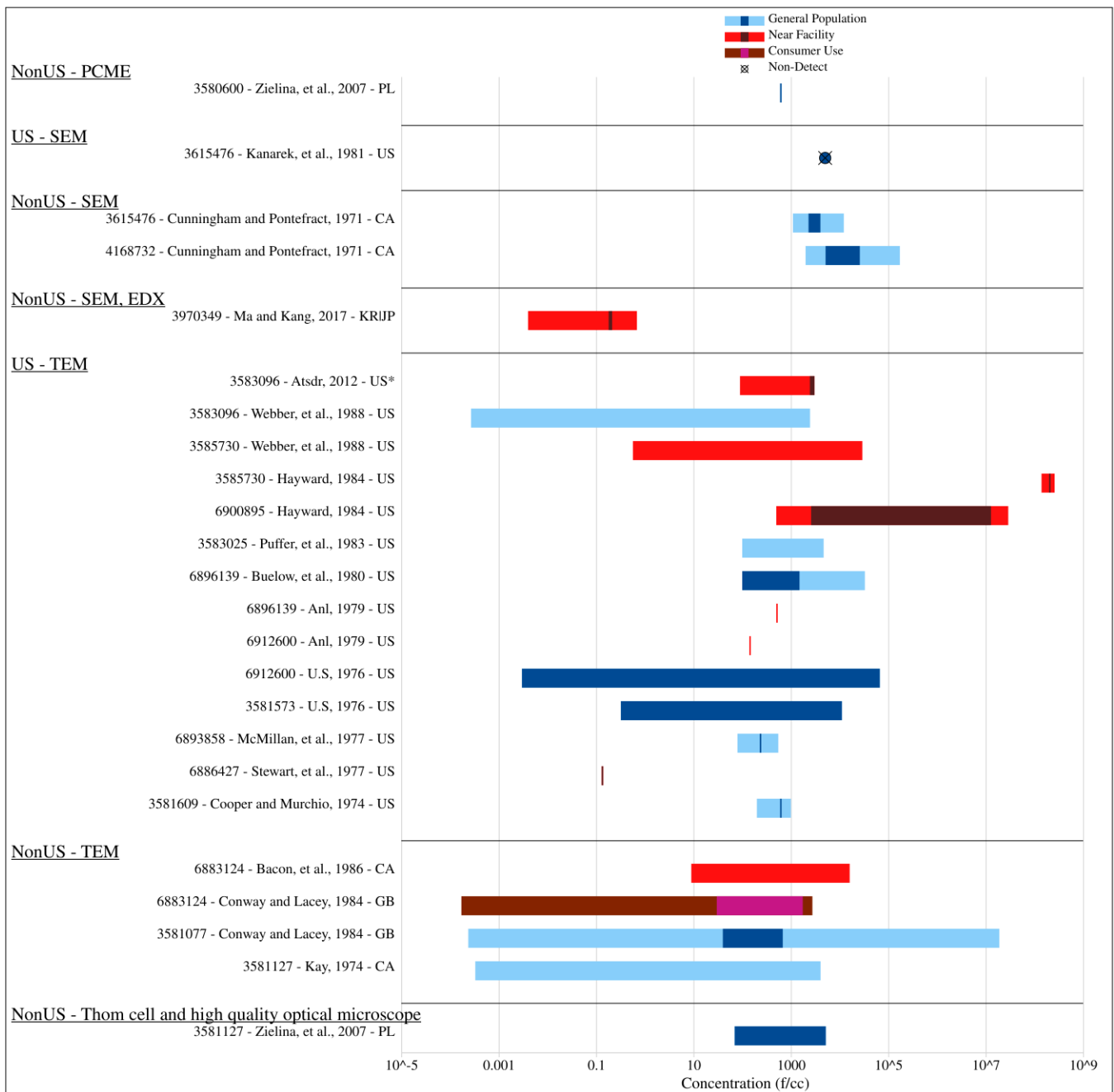
Figure_Apx F-12. Concentrations of Asbestos (f/cc) in Drinking Water from 1971 to 2011 * = Reference used in risk evaluation
