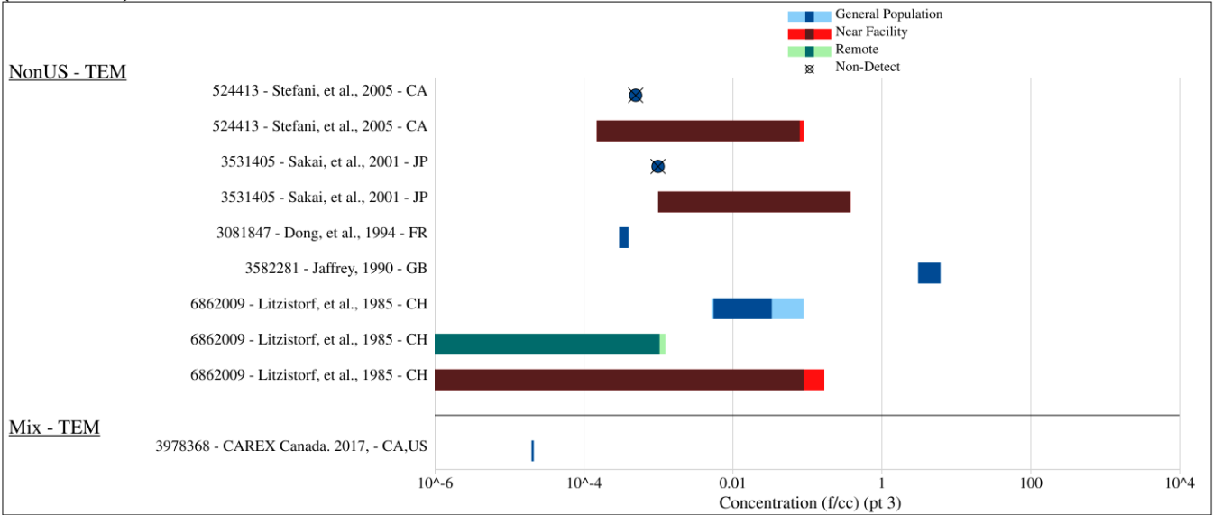
8775 Figure_Apx F-1. Concentrations of Asbestos (f/cc) in Ambient Air from 1977 to 2021
