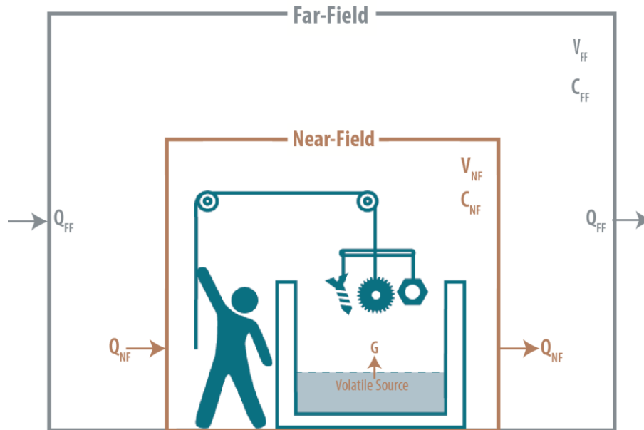
Figure_Apx P-1. Schematic of the Open-Top Vapor Degreasing Near-Field/Far-Field Inhalation Exposure Model
