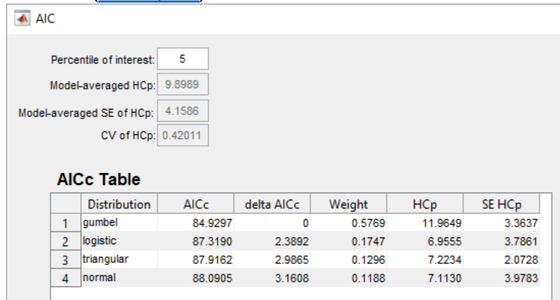
Figure_Apx E-5. AIC c for the four distribution options in the SSD Toolbox for TCE's acute hazard data (Etterson, 2019)
