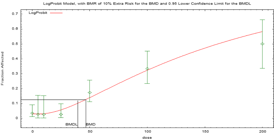
Figure_Apx F-1. Plot of Incidence by Dose (ppm) with Fitted Curve for Log-Probit Model for Mortality from Introduced Infection in Mice Following Inhalation Exposure to TCE (Selgrade and Gilmour 2010); BMR = 10% Extra Risk
