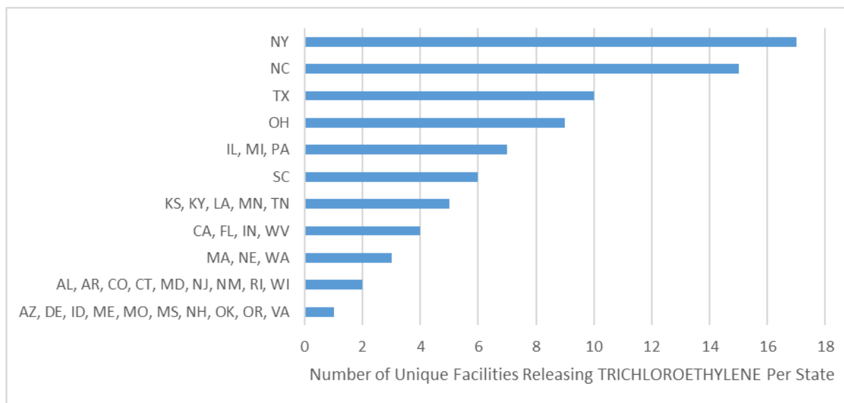
Figure 2-3. Distribution of Active Facility Releases Modeled
