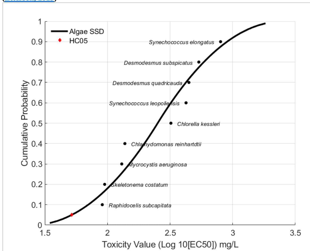
Figure_Apx E-3. TCE algae data fit with triangular distribution fit with graphical methods (Etterson, 2019)
