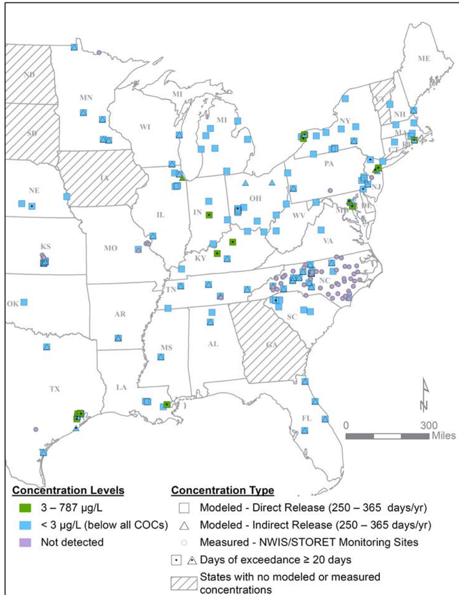
Figure 4-1. Concentrations of Trichloroethylene from Releasing Facilities (Higher Release Frequency Scenarios) and WQX Monitoring Stations: Year 2016, East US. [Note: All indirect releases are mapped at the receiving facility unless the receiving facility is unknown.]
