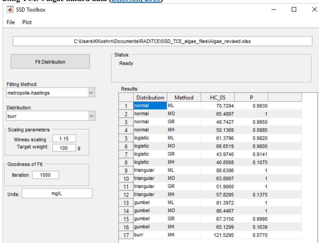
Figure_Apx E-1. SSD Toolbox interface and list of HC 05 s for each distribution and fitting method using TCE's algae hazard data (Etterson, 2019)
