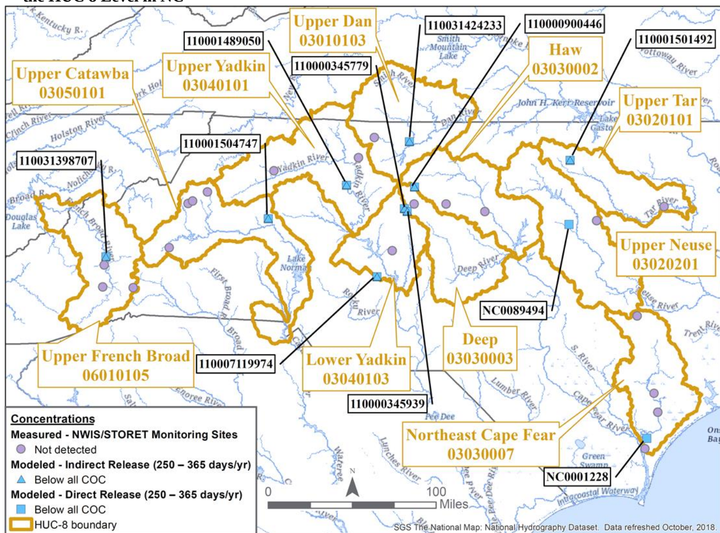
Figure 4-5. Co-location of Trichloroethylene-Releasing Facilities and WQX Monitoring Stations at the HUC 8 Level in NC
