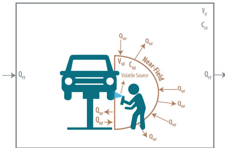
Figure_Apx L-1. The Near-Field/Far-Field Model as Applied to the Brake Servicing Near-Field/Far-Field Inhalation Exposure Model
