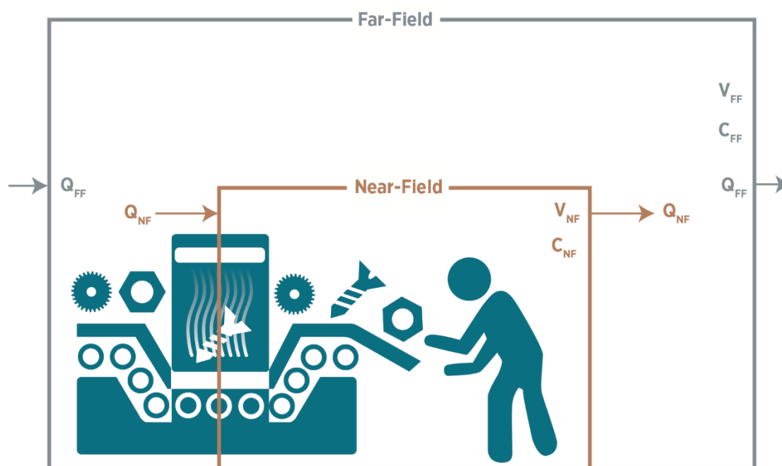
Figure_Apx P-2. Belt/Strip Conveyorized Vapor Degreasing Schematic of the Conveyorized Degreasing Near-Field/Far-Field Inhalation Exposure Model
