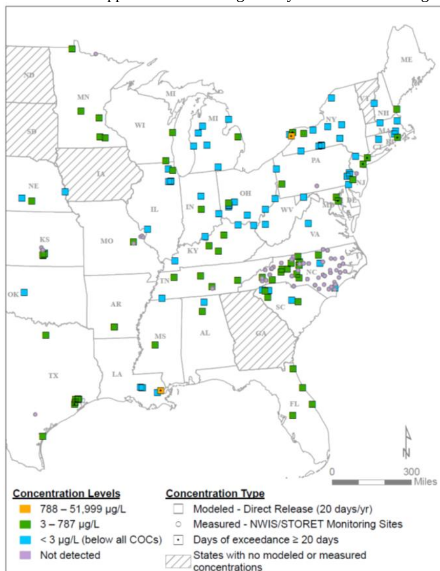
Figure 4-3. Concentrations of Trichloroethylene from Releasing Facilities (20 Days of Release Scenario) and WQX Monitoring Stations: Year 2016, East US.
