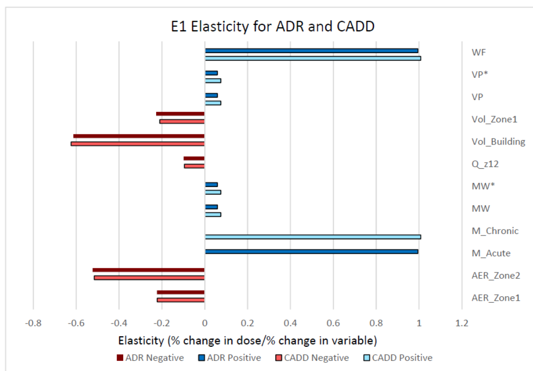
Figure_Apx D-1. Elasticities ( \geq 0.05 ) for Parameters Applied in E1
