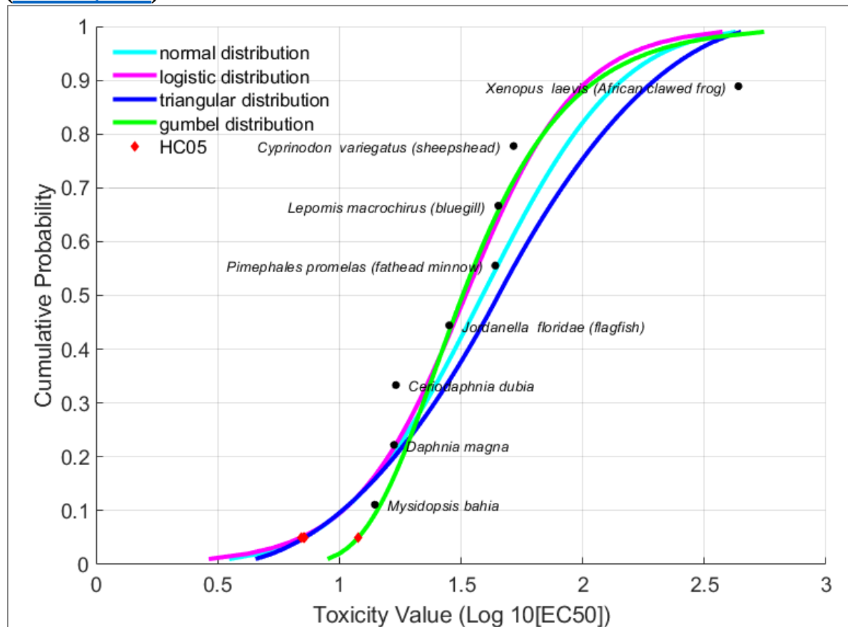
Figure 3-2. Species Sensitivity Distributions (SSDs) for Acute Hazard Data Using LC 50 s or EC 50 s (Etterson, 2019)
