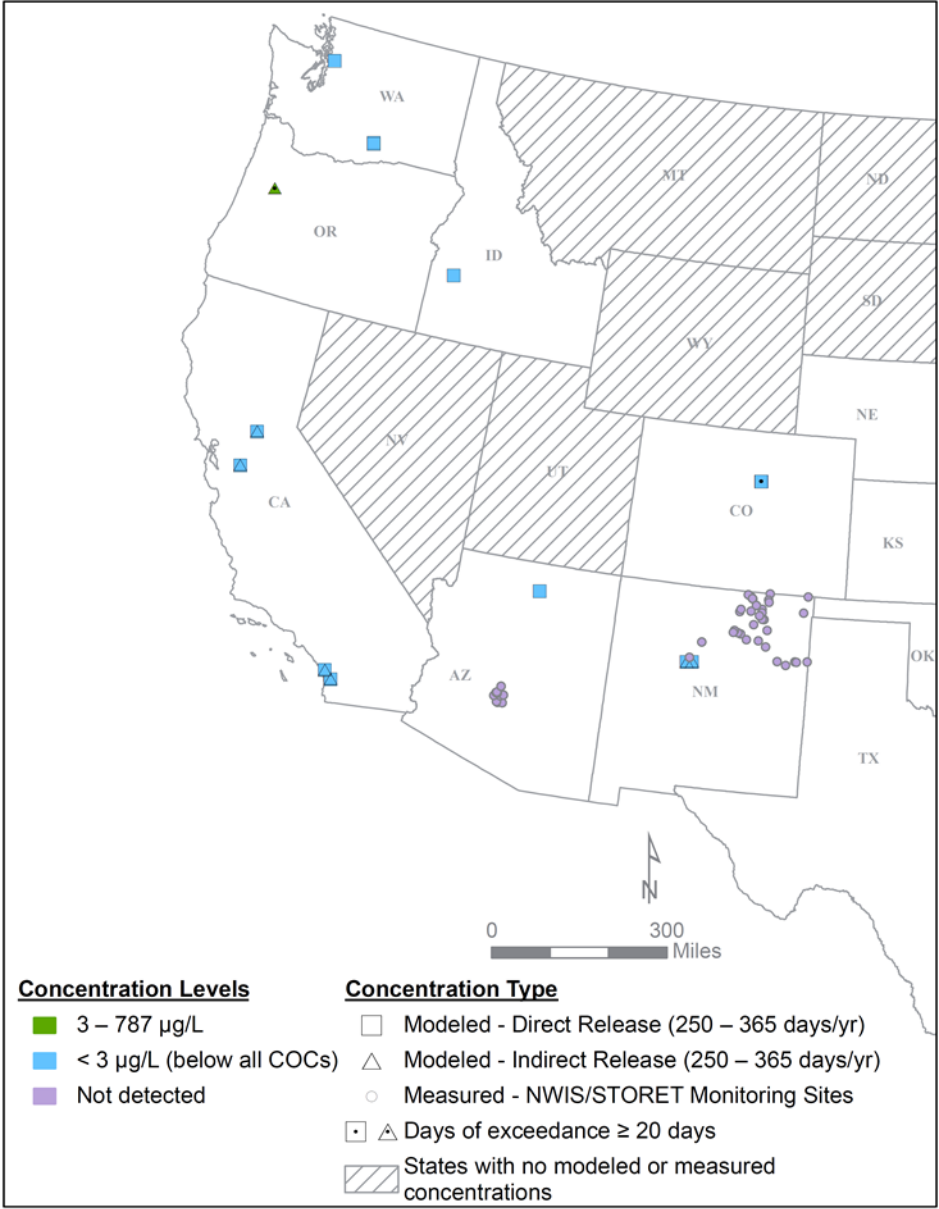
Figure 4-2. Concentrations of Trichloroethylene from Releasing Facilities (Higher Release Frequency Scenarios) and WQX Monitoring Stations: Year 2016, West US. [Note: All indirect releases are mapped at the receiving facility unless the receiving facility is unknown.]
