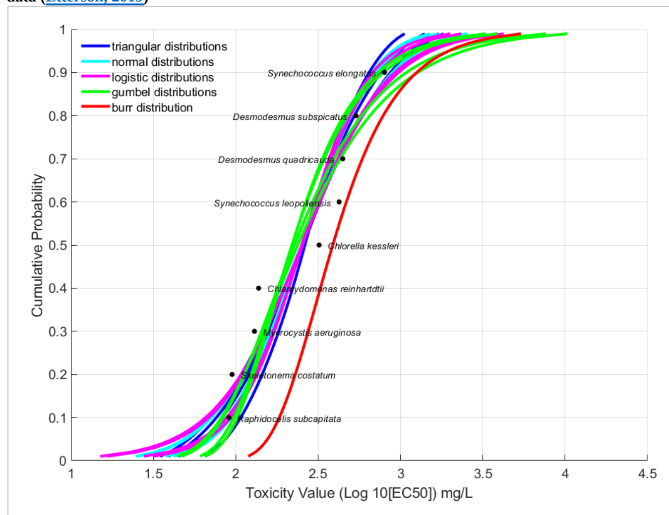
Figure_Apx E-2. All distributions and fitting methods in the SSD Toolbox for TCE's algae hazard data (Etterson, 2019)
